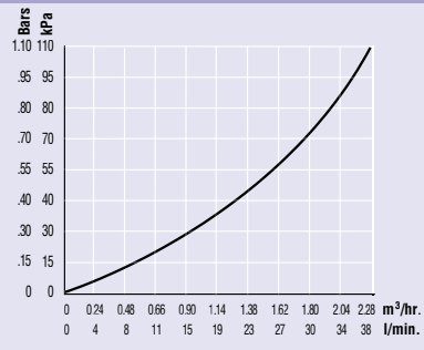
Swing Joint Friction Loss – Metric
