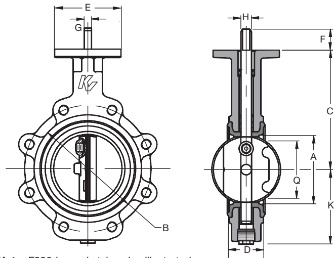
Note: F222 lugged style valve illustrated
