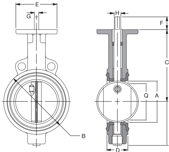
Note: F221 Wafer style valve illustrated
