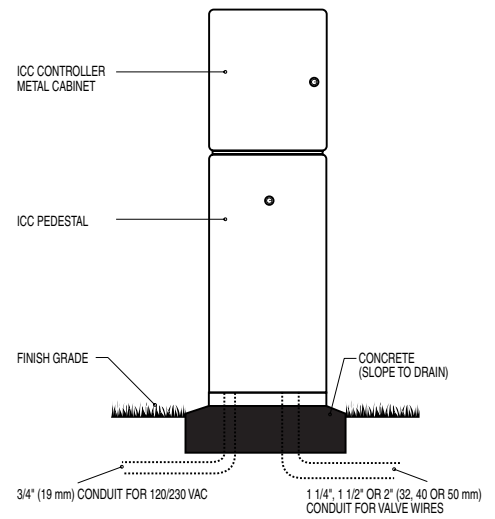
Hunter® ICC-PED
