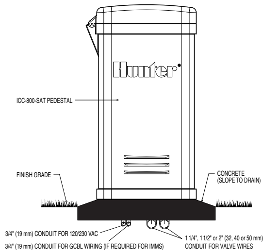
Hunter® ICC-PLASTIC-PED
