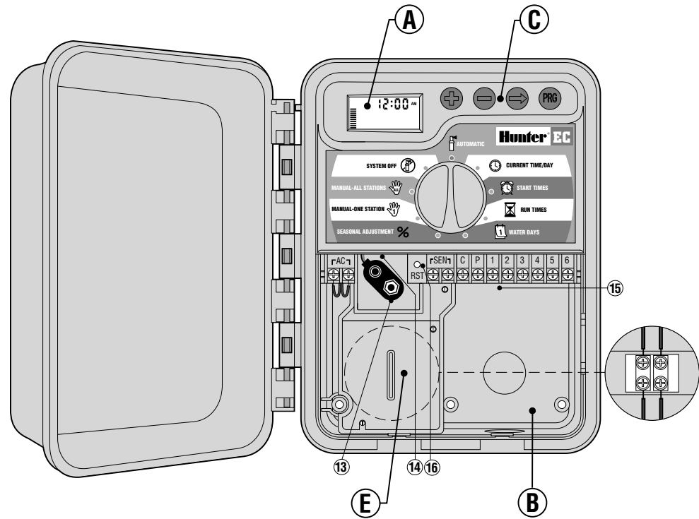
Outdoor Model (Internal Transformer Included)
