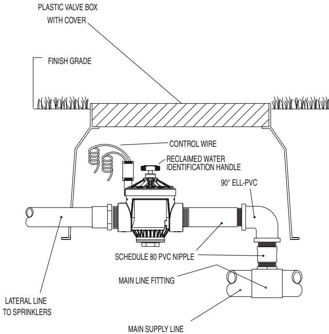
Hunter® 2" PGV-NP
