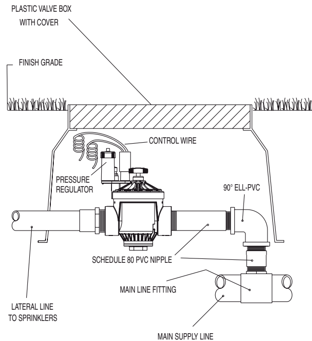
Hunter® 2" PGVW/PR
